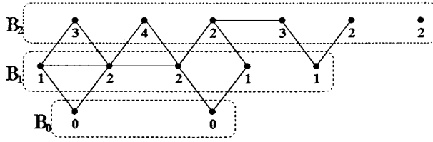
FIG. 1. Illustration of the progression of the boundary B . Each dot corresponds to a substring. The number associated with dot x is W_v[x] . Arcs connect neighboring substrings.
